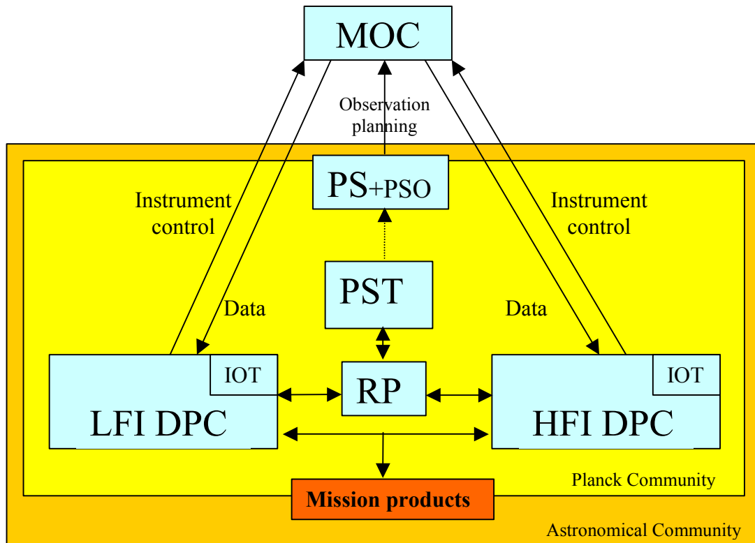
Figure 1. A schematic view of the various elements supporting Planck during its operational phase, and the flow of data and information among them. DPC stands for Data Processing Center (see Section 2.2), and RP for Reflector Provider. Each instrument is operated by a dedicated Instrument Operations Team (IOT). The Planck Science Office (PSO) directs the scientific operations, e.g. survey coverage.
